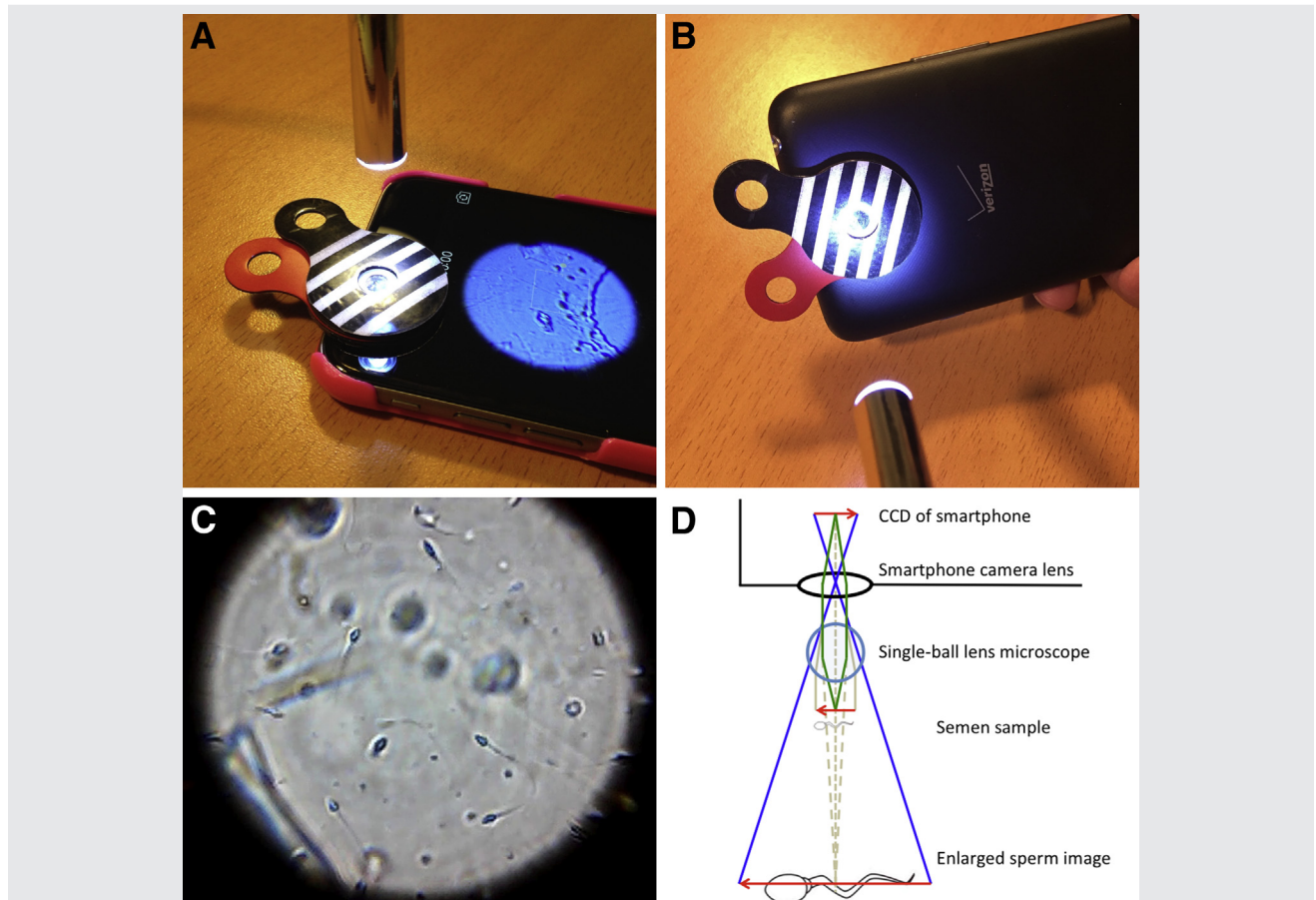
(A) The mobile phone microscopy apparatus with an 0.8-mm ball lens enveloped in a plastic jacket and attached to the iPhone 6s FaceTime camera. (B) The technique for observing semen sample using a ball lens and LG Optimus Exceed 2 with a single light-emitting diode flashlight providing illumination. (C) The sperm could be observed clearly with a ball lens and iPhone 5s. (D) Diagram of this ball lens and smartphone camera.
